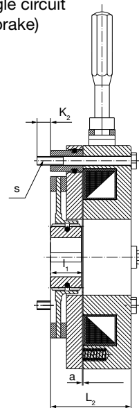
Type 896.105.33 (Single circuit brake)
