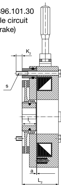
Type 896.105.33 (Single circuit brake)
