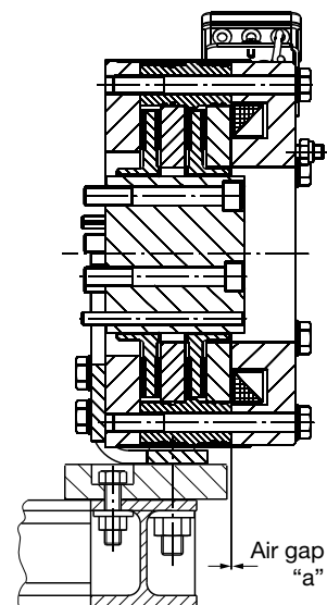
Type 896.8 _ _ .11 (Double rotor design)
