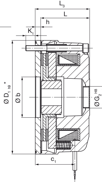
Type 891.414.1 Enclosed design (IP 65) with flange plate
