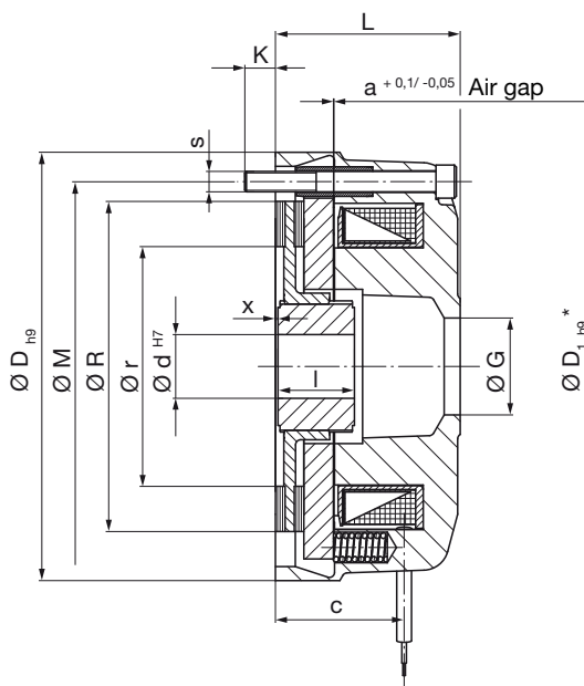
Type 891.410.0 Standard, enclosed
